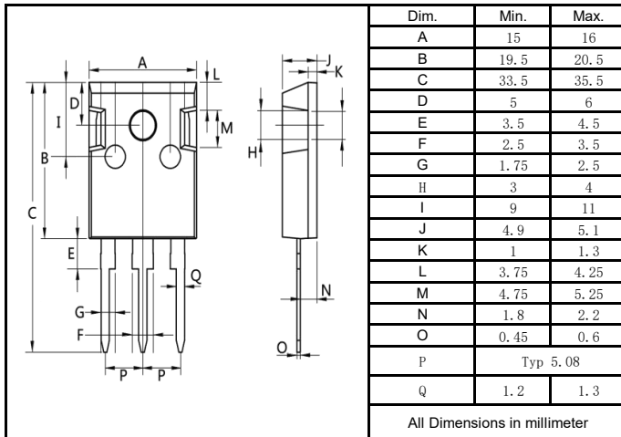
T0-247S
